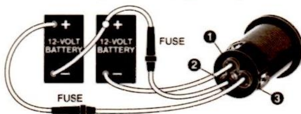
12/24V (also 24/36V) Configuration (Figure 4)
